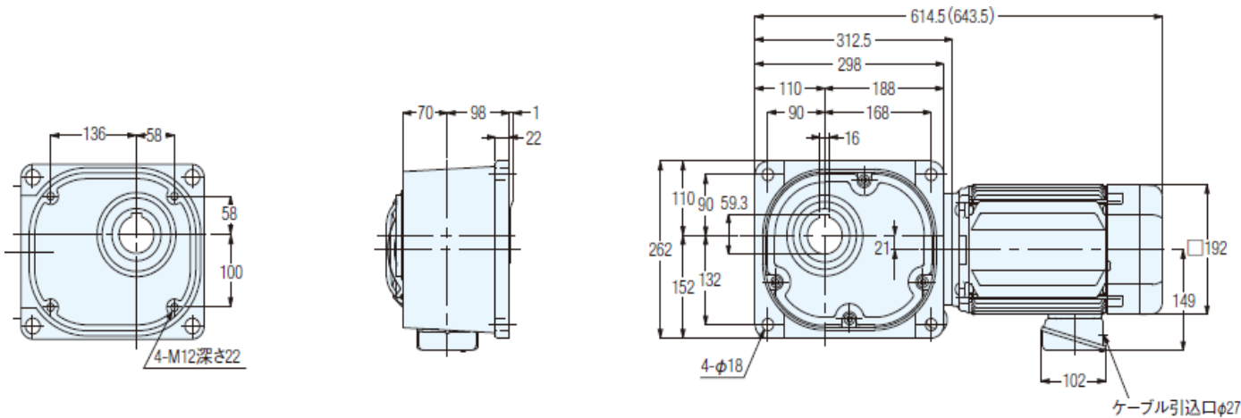
F Series 2.2kW Frame55 Ratio: 1/40-1/120
